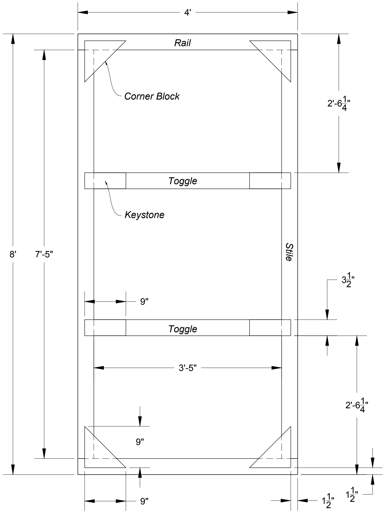
Traditional Flat Diagram w/ Labels Scale: 0'-1"=1'-0"
