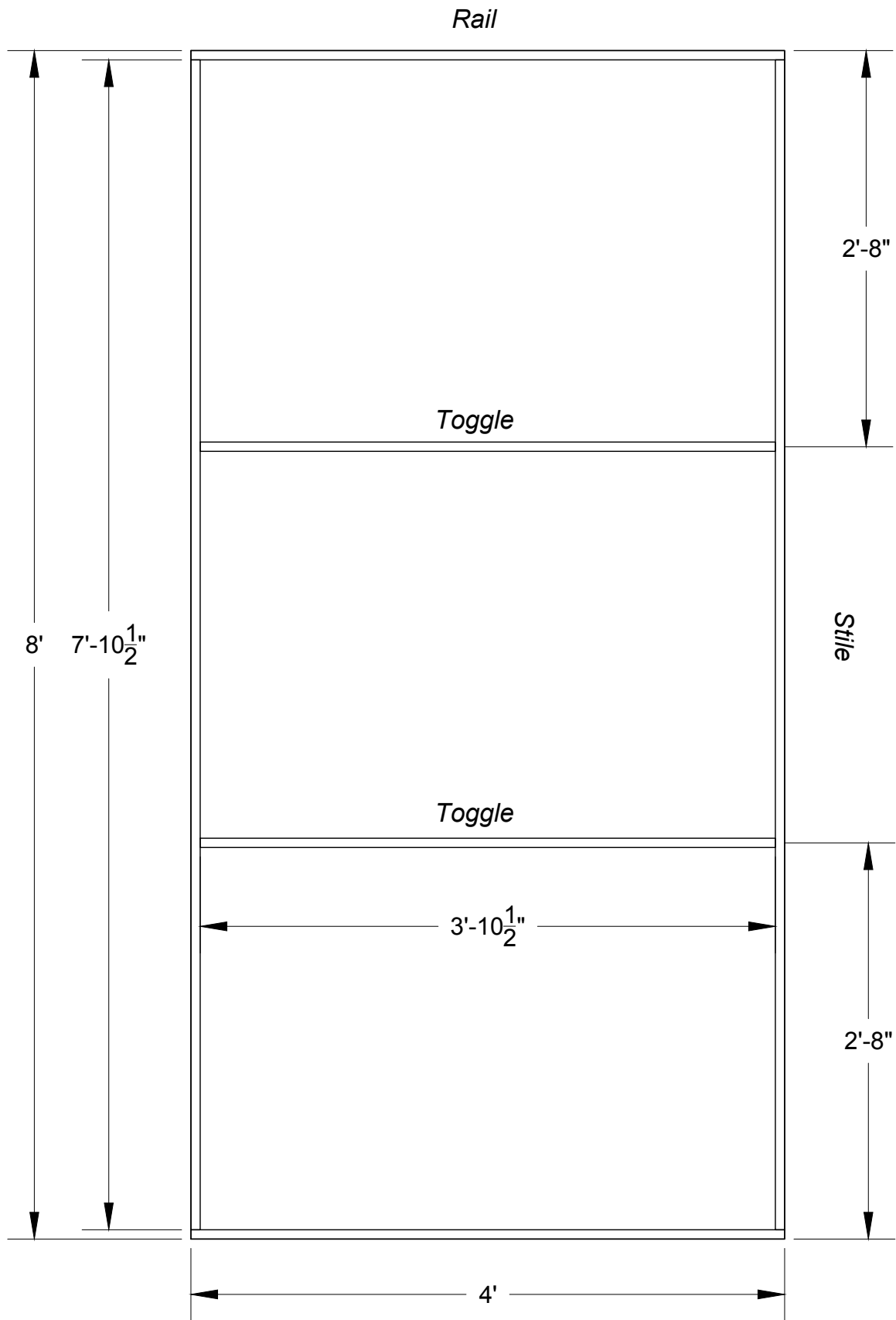
Hollywood Flat Diagram w/ Labels Scale: 0'-1"=1'-0"
